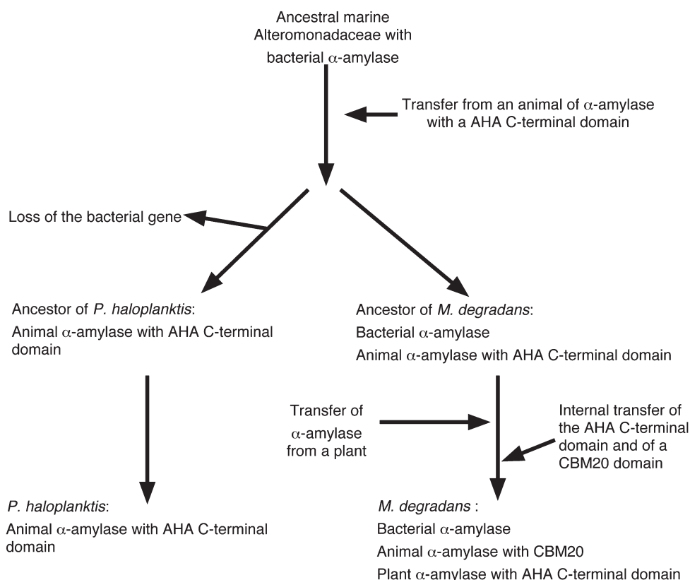
Figure 5. A scenario, among several, for the evolution of \alpha -amylases in Pseudoalteromonas haloplanktis and its relative Microbulbifer degradans ( \gamma -proteobacteria: Alteromonadaceae).
